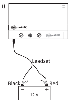
12 volt battery via the leadset
